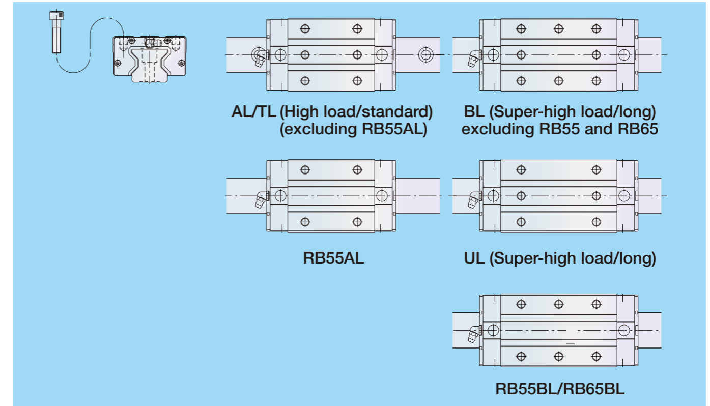
Fig. 5 Flanged type
